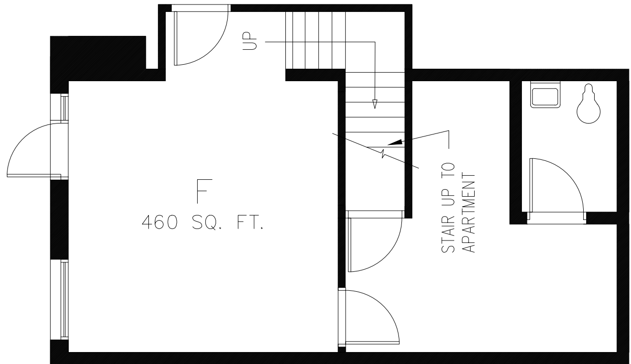
SUITE F FLOOR PLAN
