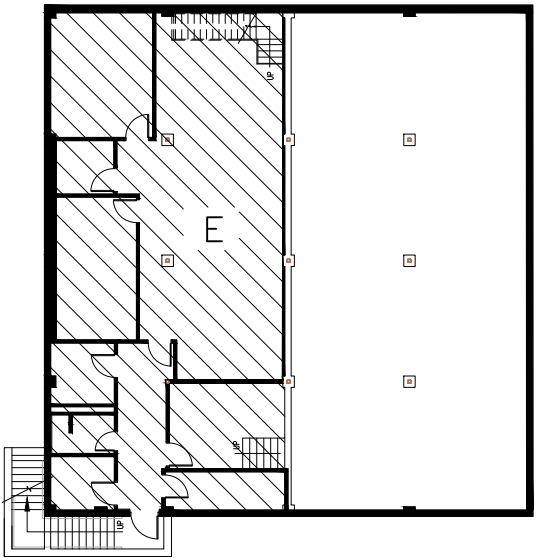
LOWER KEY PLAN
